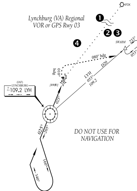
Figure 6-8 Sample Approach with Procedure Turn
