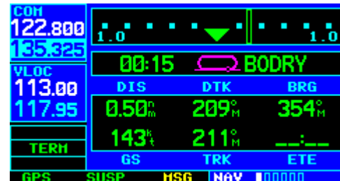
Figure D-3 'SUSP' Annunciation
