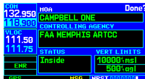
Figure 8-35 Airspace Page for MOA
