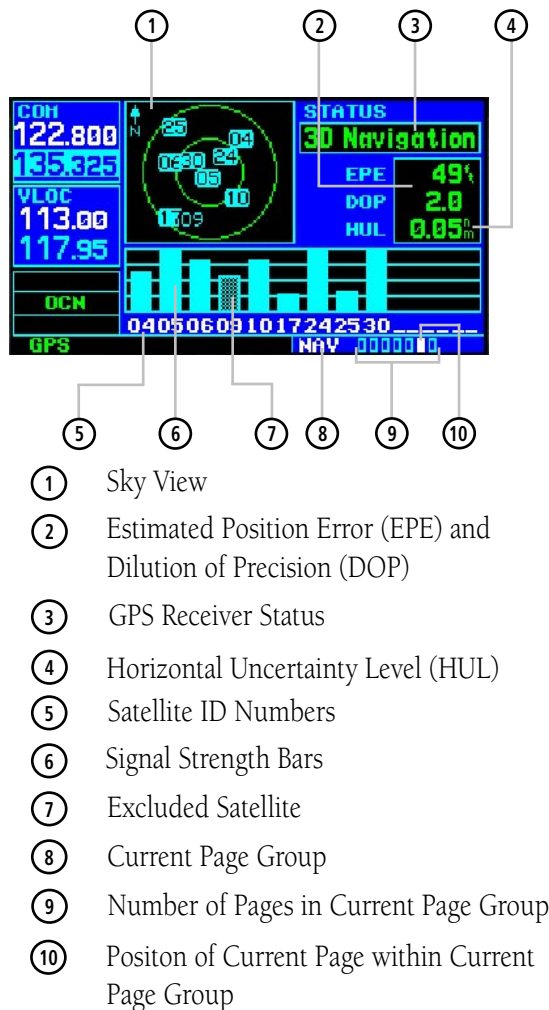
Figure 3-46 Satellite Status Page
