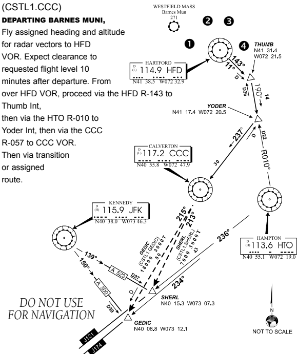
Figure 6-68 Coastal One Departure
